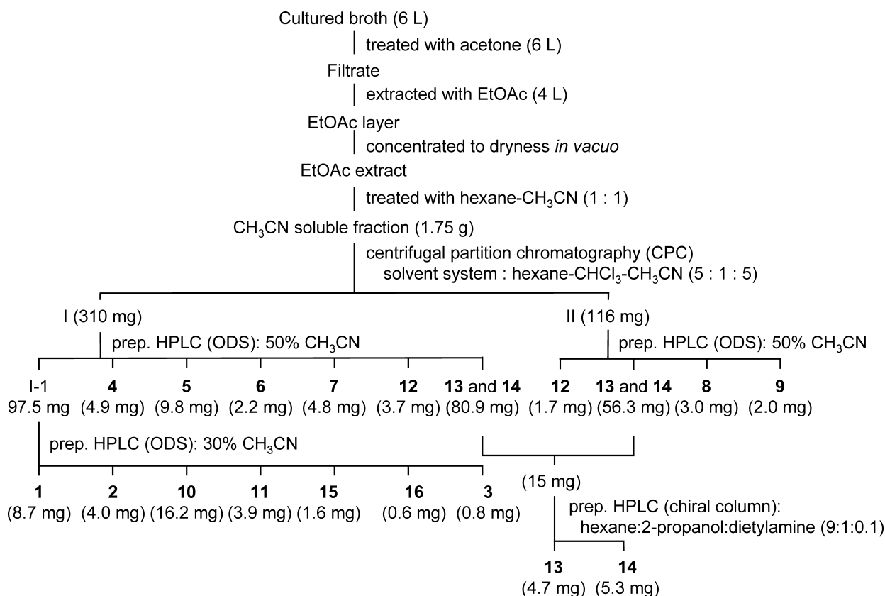
Fig. 3 Procedure for purification of yaequinolones and related compounds from the culture broth of Penicillium sp. FKI-2140.
